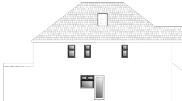
PROPOSED SIDE ELEVATION A
