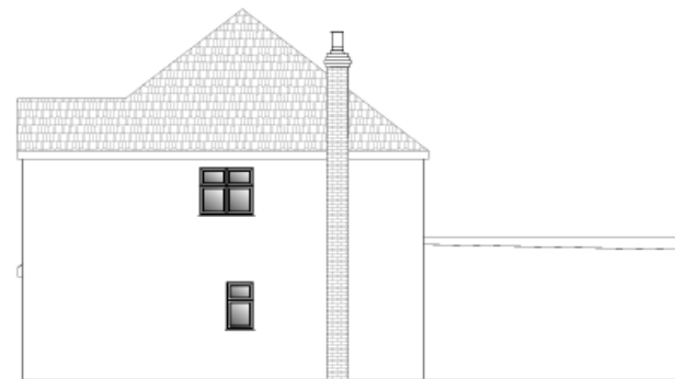
EXISTING SIDE ELEVATION B
